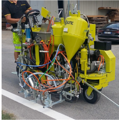
Airless machines with hydraulic drive
